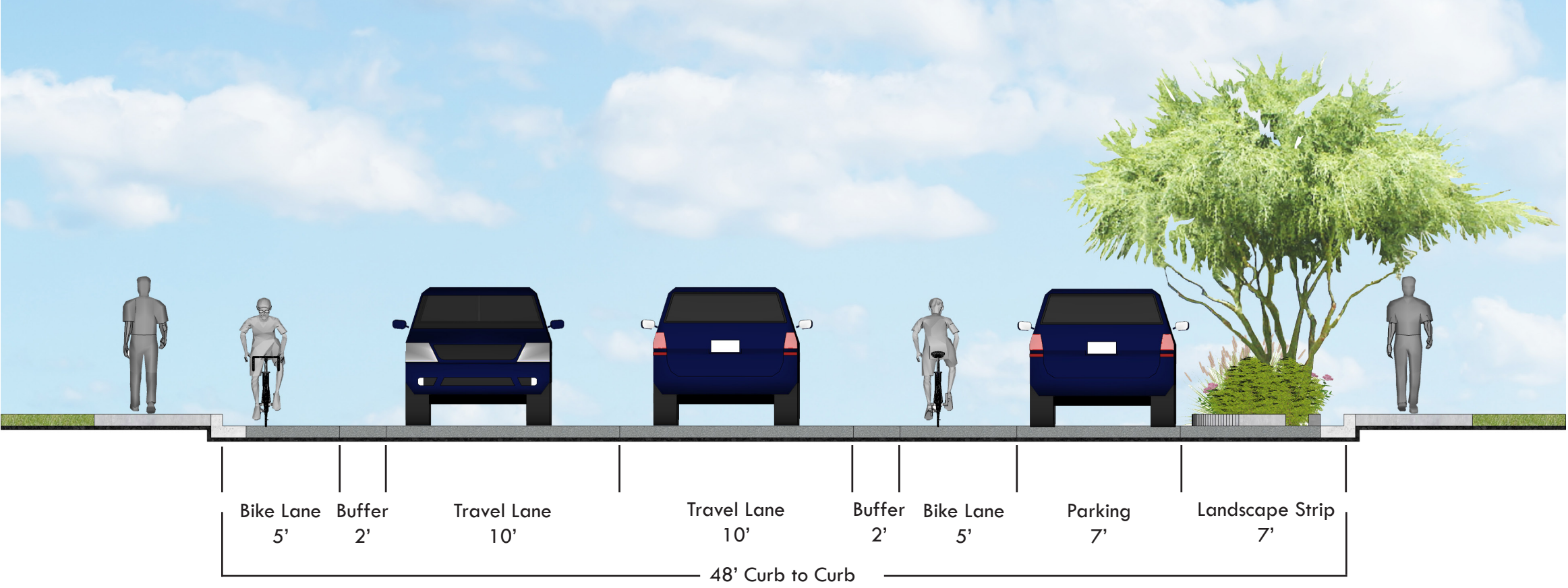
Mill Avenue to College Avenue - Typical Section
