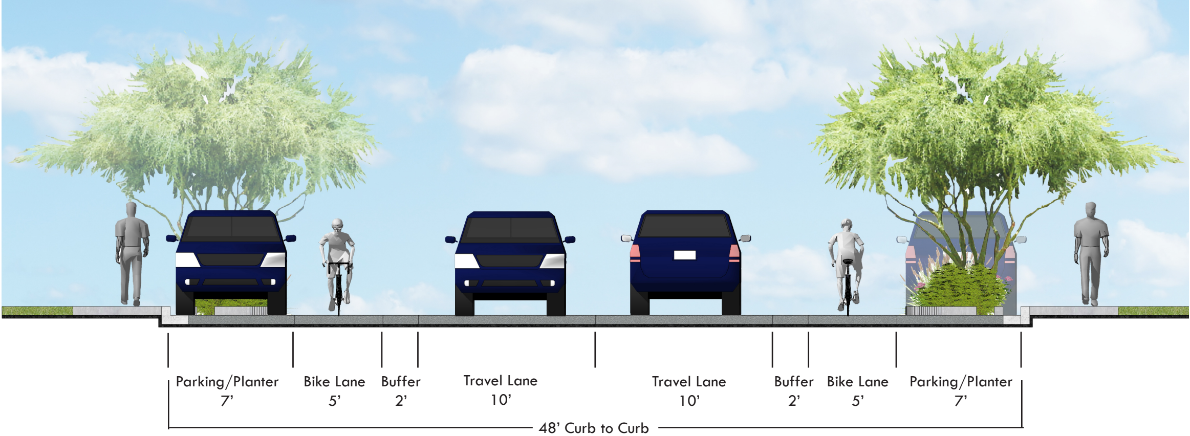
Railroad to Mill Avenue - Typical Section
