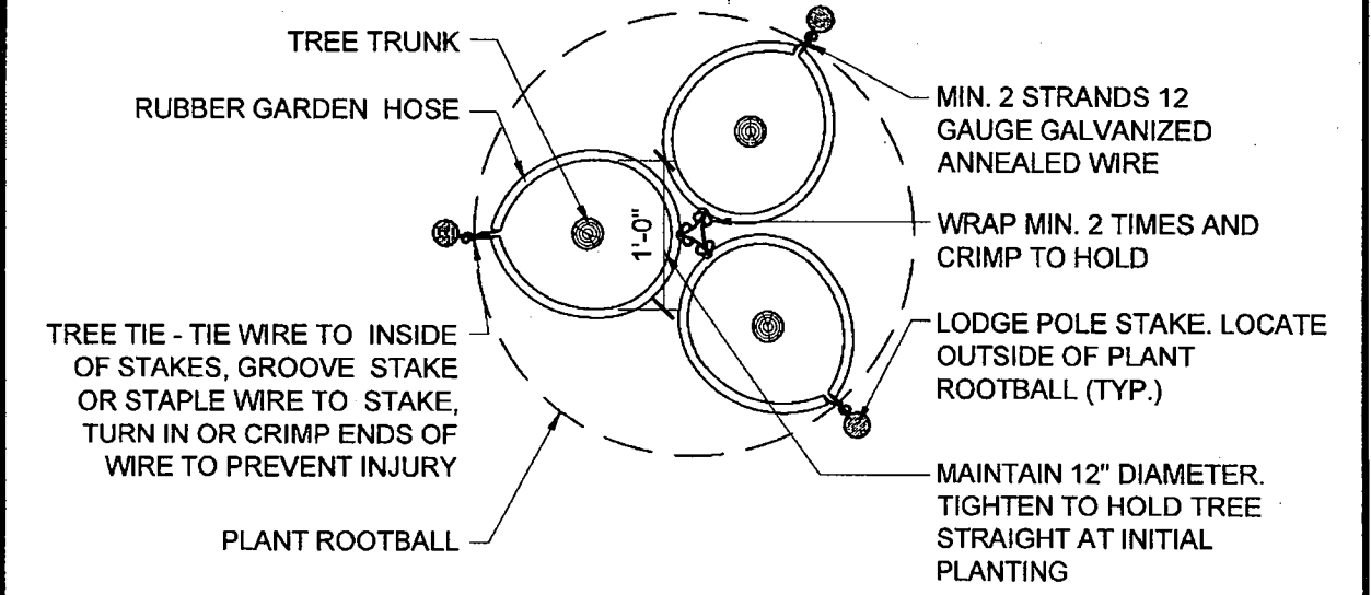
TREE STAKING PLAN - TRIPLE
