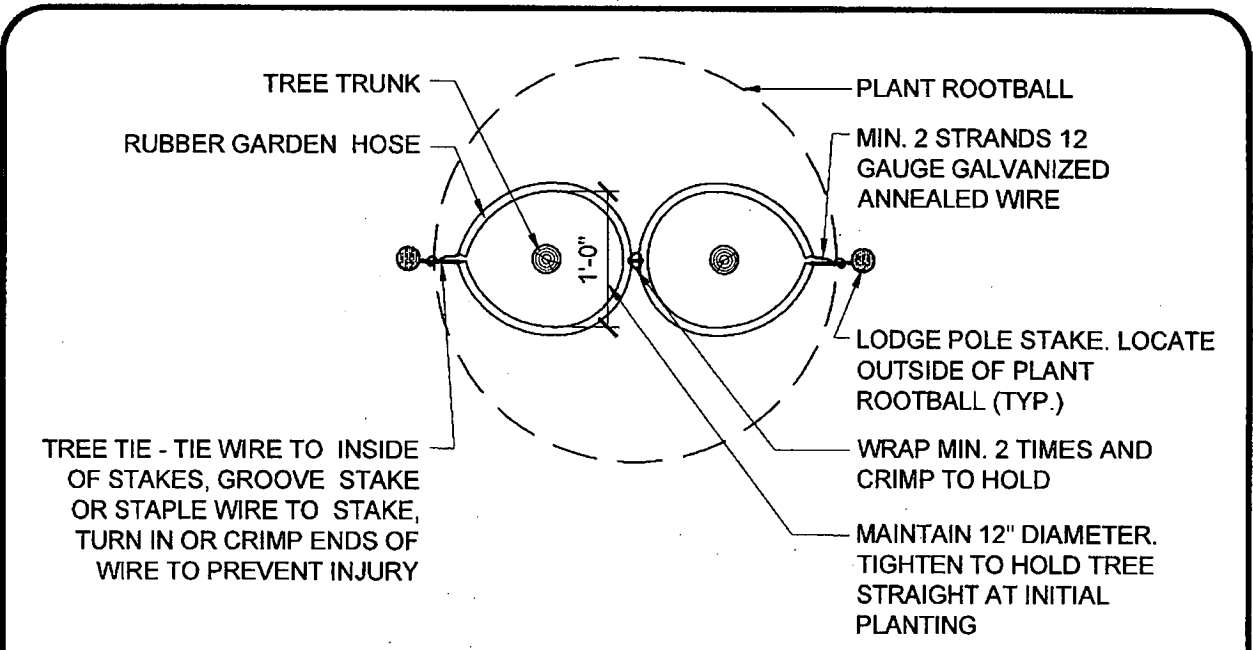
TREE STAKING PLAN - DOUBLE
