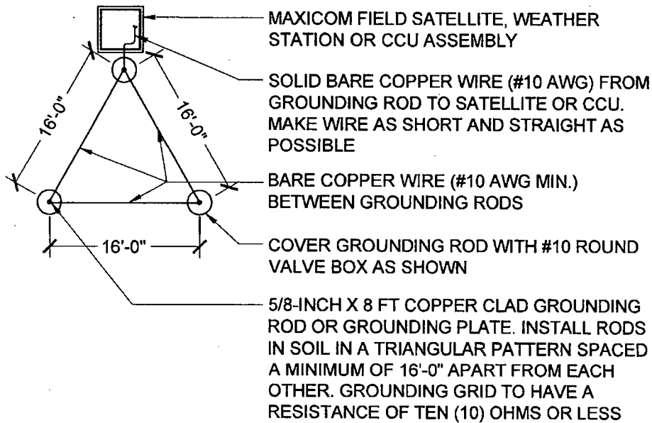
GROUND ROD LAYOUT
