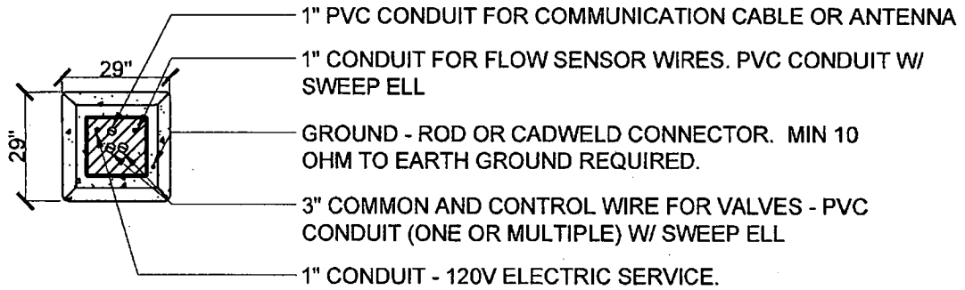
PEDESTAL MOUNTING CONCRETE PAD (PLAN VIEW)
