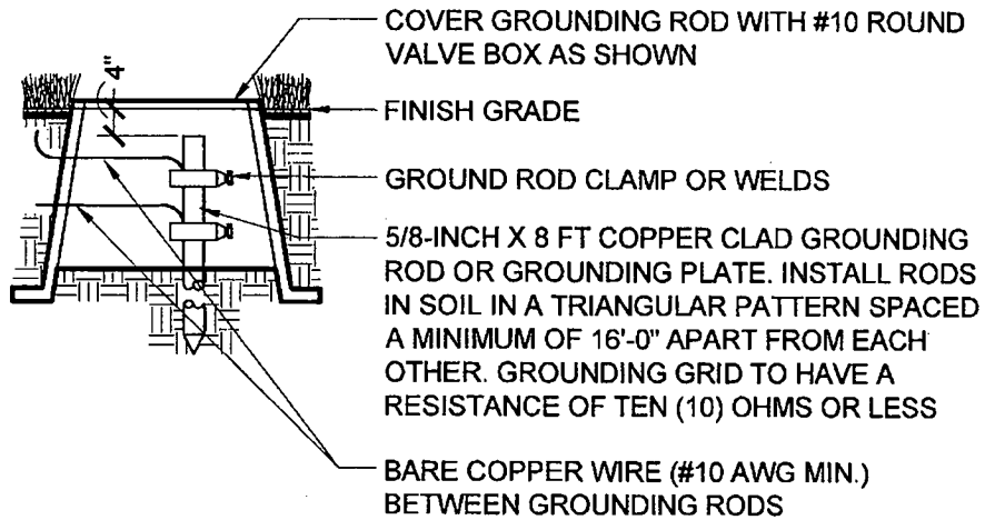
GROUND ROD ASSEMBLY
