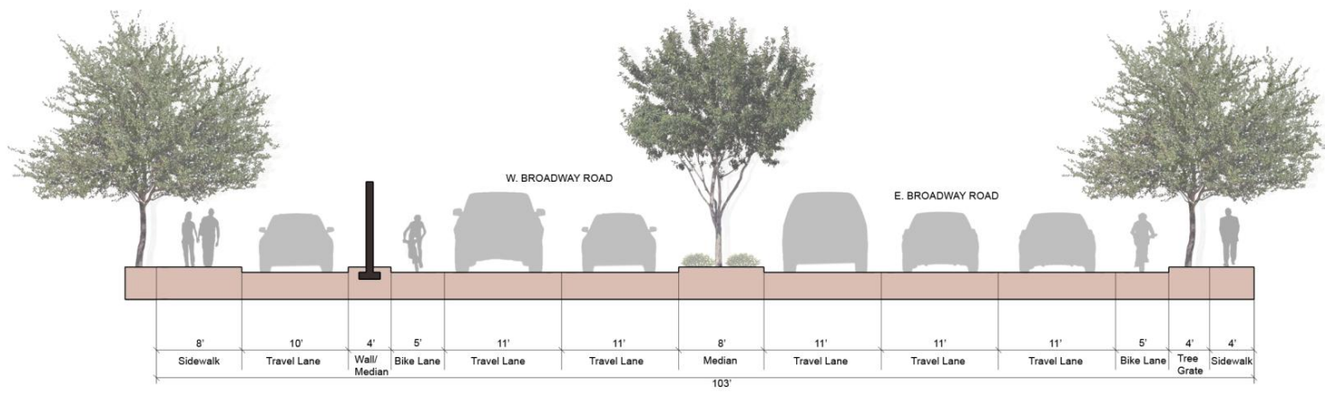
BROADWAY ROAD CROSS SECTION
