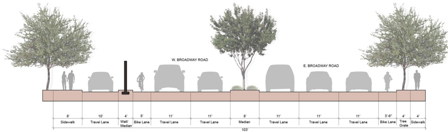
BROADWAY ROAD CROSS SECTION
