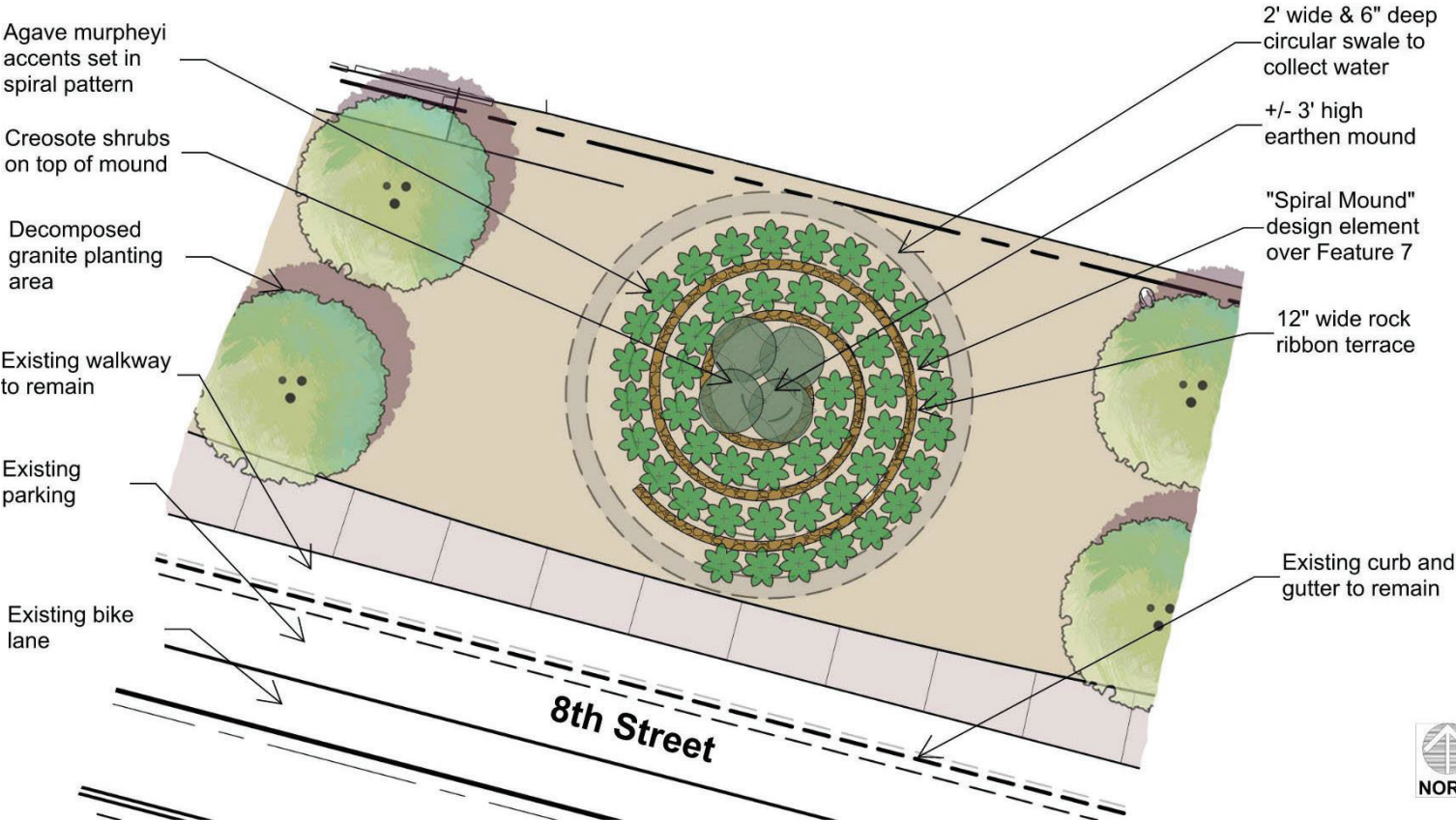
6007131B - Multi-Use Path - 8th Street; Rural Road to McClintock Dr. Feature 7 - Spiral Mound Concept Date: 09.14.2023
